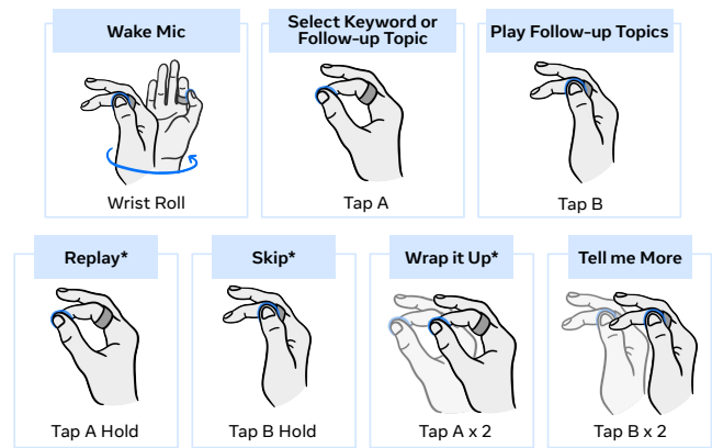
Figure 12: Mapping of Gestures to System Functions. For our user study, we designed a gesture set leveraging three distinct poses (Wrist Roll, Tap A, Tap B) with variations of the tap gestures (holding or repeated taps) to distinguish between system functions. This mapping is a simplified version of the gesture set described in Sec. 3. (*) indicates gestures introduced in Task 2.
